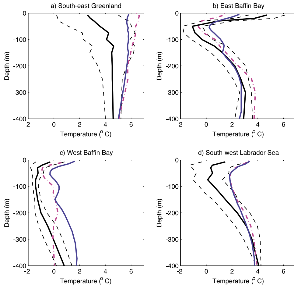
Figure 4 The 2004–8 annual mean temperature profiles at the 4 locations ( 1^\circ grid cells) of the North-West Atlantic shown in Figure 2a); a) South-east Greenland ( 39.5^\circ\text{W} , 63.5^\circ\text{N} ), b) East Baffin Bay ( 57.5^\circ\text{W} , 70.5^\circ\text{N} ), c) West Baffin Bay ( 64.5^\circ\text{W} , 68.5^\circ\text{N} ), d) South-west Labrador Sea ( 58.5^\circ\text{W} , 56.5^\circ\text{N} ): ATLAS (black solid line) with associated OA error (black dashed line); EN3 (solid blue line) and L09 (dashed magenta line).
