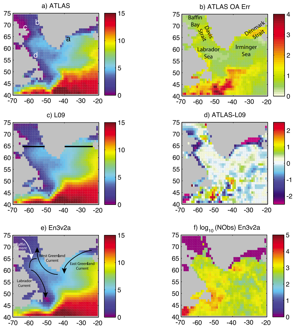
Figure 2 Maps showing the 2004–08 annual mean temperature ( ^{\circ}\text{C} ) averaged over 0–500 m for a) ATLAS, c) L09 and e) EN3. b) OA error ( ^{\circ}\text{C} ) for the ATLAS temperature field shown in Figure 2a. d) The difference, ATLAS - L09, of the temperature fields shown in Figures 2a and 2c. f) The number of observations (top 500 m) used in EN3 on a \log_{10} scale. The letters in Figure 2a refer to profiles examined in Figure 4 and the section shown in Figure 2c is that used in Figure 3. The key boundary currents are shown schematically in Figure 2e.
