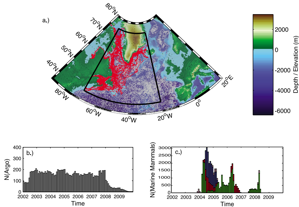
Figure 1 a) Distribution of temperature profiles from Argo (grey dots) and marine mammal-mounted sensors (red dots). Monthly number, N , of b) Argo and c) marine mammal (hooded seals, green; harp seals, red; grey seals, blue; beluga, pink) profiles in the study area (black box in Figure 1a).
