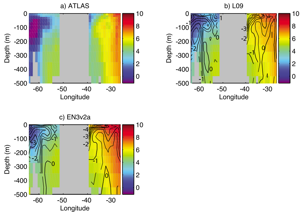
Figure 3 Coloured field: Longitude–depth section of 2004–08 annual mean temperature ( ^{\circ}\text{C} ) at 64.5^{\circ}\text{N} for a) ATLAS, b) L09 and c) EN3. Contours show the difference of these fields for Figure 3b, ATLAS - L09, and Figure 3c, ATLAS - EN3, contour intervals 0.5^{\circ}\text{C} , integer contour values are labelled. To aid comparison, EN3 was re-gridded on to the ATLAS grid.
